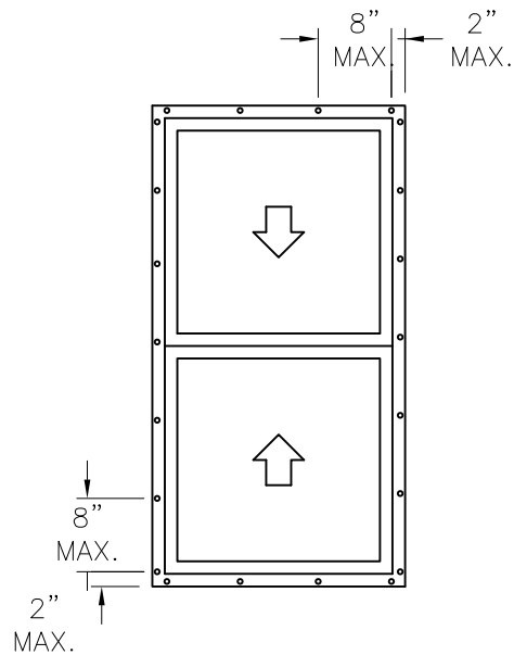
Elevation View
